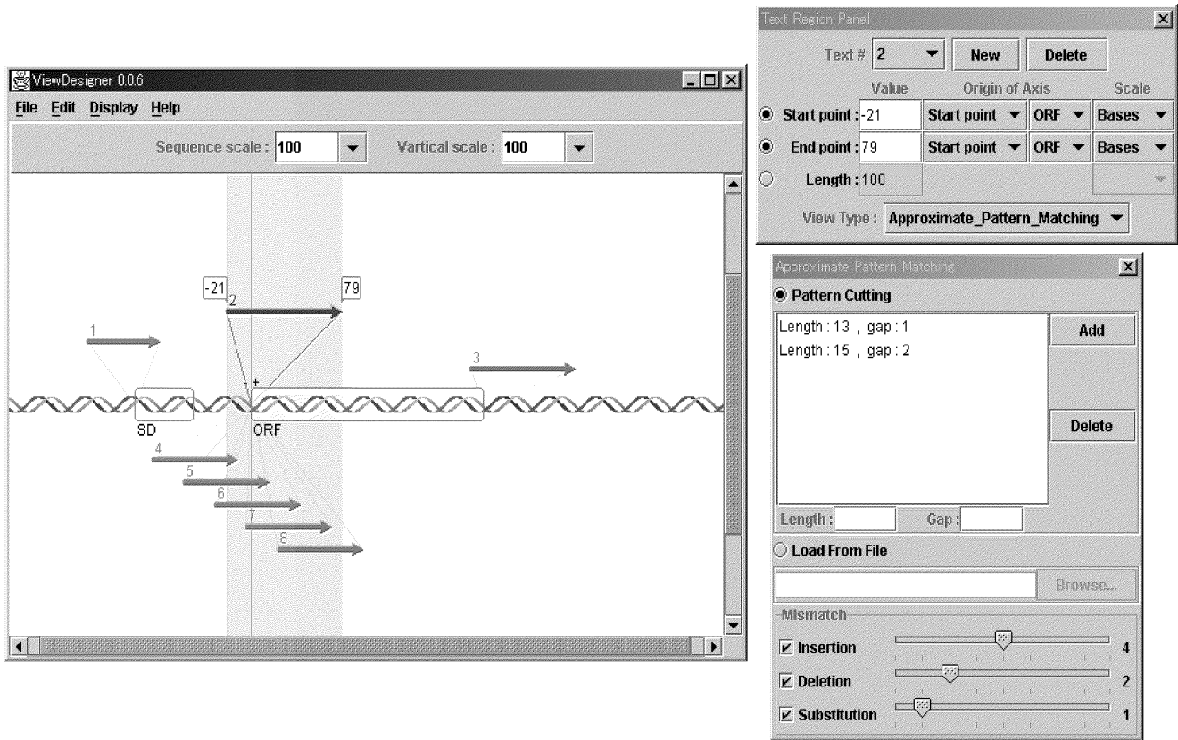
Figure 1: VIEWDESIGNER
