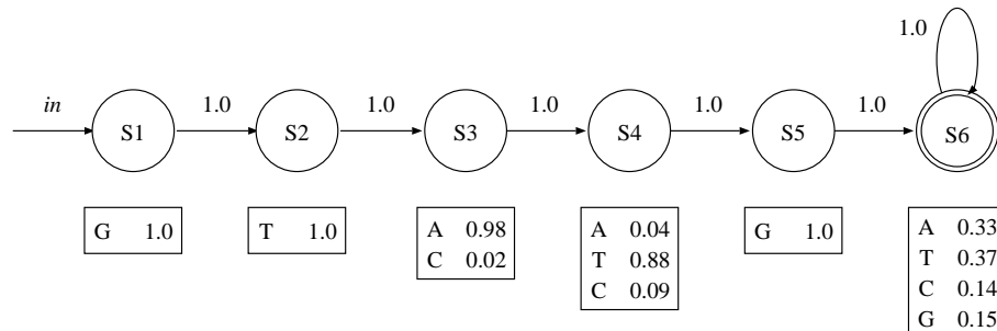
Figure 2: An HMM obtained using the method
